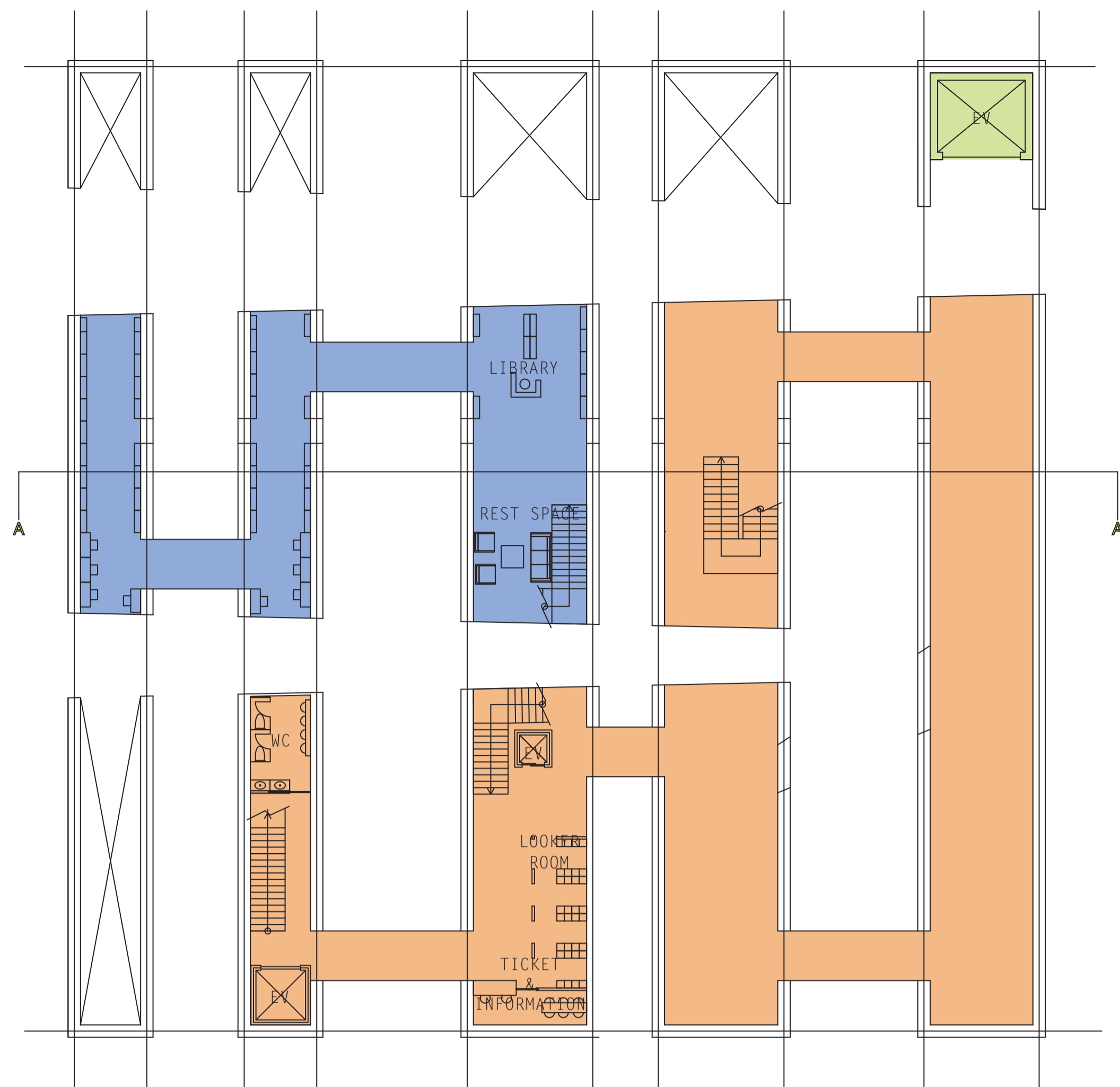
2F PLAN 1/100
