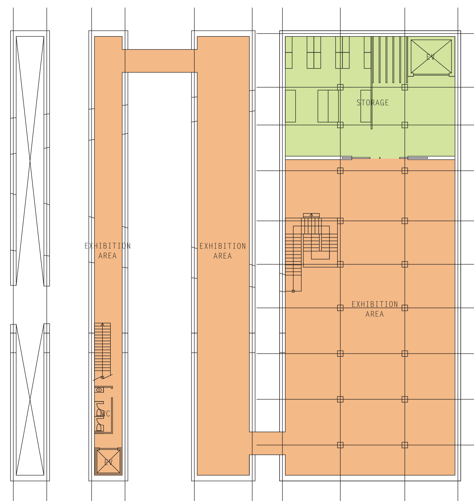
3F PLAN 1/100
